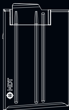
10rd metal magazine 6,5x47 Lapua, 6,5 CM, 308 Win
